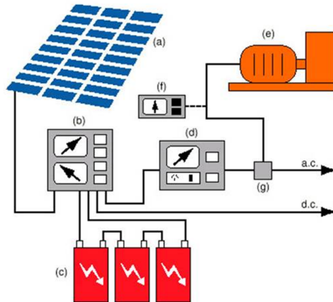
BIPV system diagram Courtesy of Murdoch University Energy Research and Innovation Group
